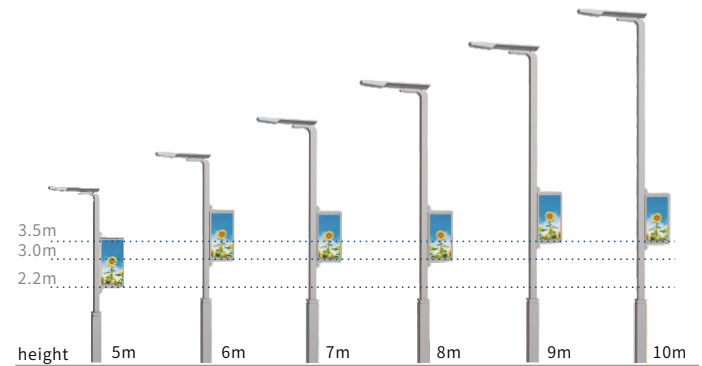
Installation Height Reference Table for 640×1280mm Light Pole Screens
