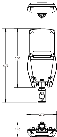
UNI-STC3-2(40-60W) UNI-STC3-3(90W)
