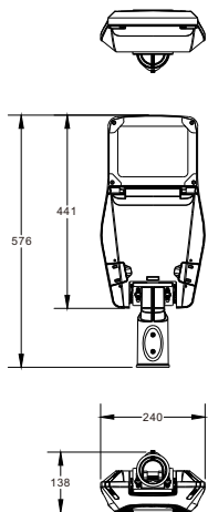
UNI-STC3-1(20-60W)
