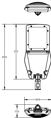
UNI-STC3-5(180-240W)
