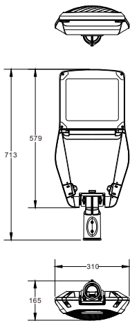
UNI-STC3-4(120-150W)
